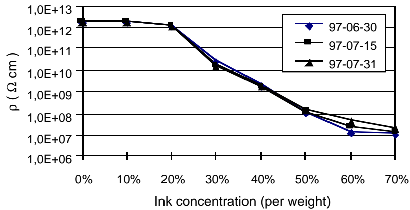
Figure 3 - The anodic material resistivity can be controlled by the amount of ink and varied from 2 \times 10^7 to 3 \times 10^{12} \Omega \text{cm} . Successive measurements taken at two weeks intervals suggest a good stability of the bulk resistivity.
