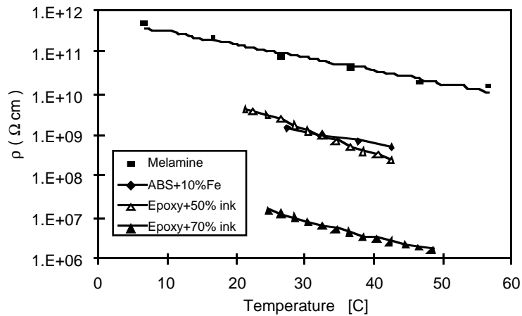
Figure 6 - Resistivity measurements performed for various materials in a temperature range of practical interest.
