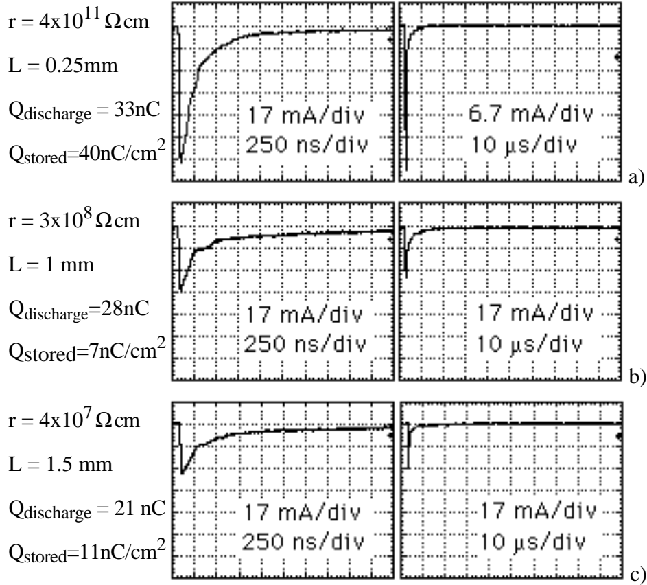
Figure 10 - Typical oscilograms of the discharge current for the anode plates studied in 2 different time scales. The quantities listed to the left of the oscilograms are: plate DC resistivity ( r ), plate thickness ( L ), observed discharge charge ( Q_{\text{discharge}} ) and charge stored in the plate capacitor per unit area ( Q_{\text{stored}} ).
